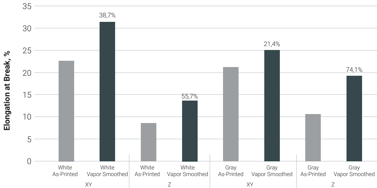
Figure 7: Elongation at Break Comparison
