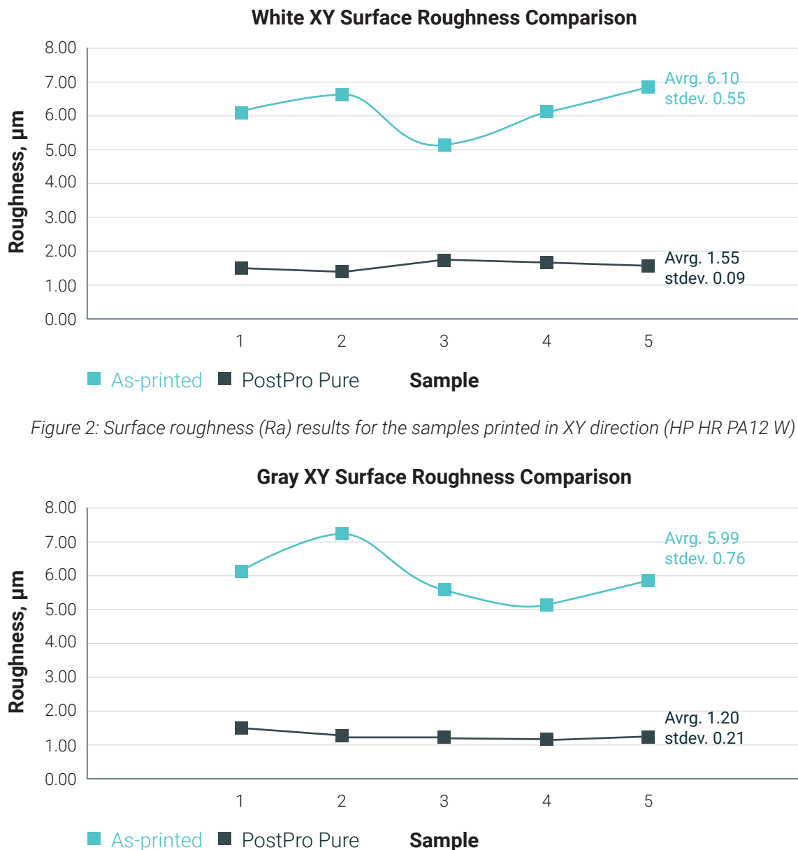
Figure 3: Surface roughness (Ra) results for the samples printed in XY direction (HP HR PA12)
