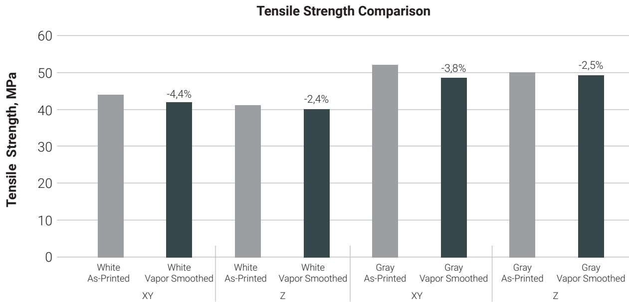
Figure 5: Tensile Strength Comparison
