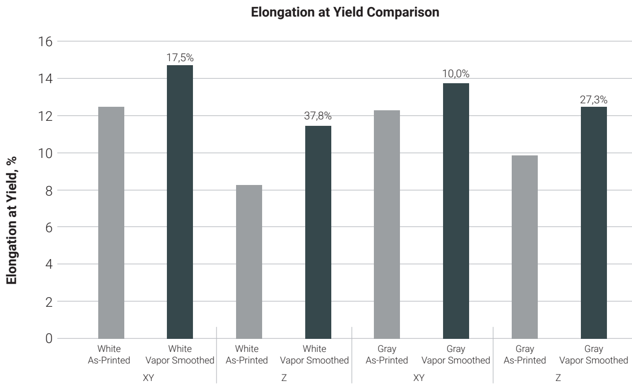
Figure 6: Elongation at Yield Comparison
