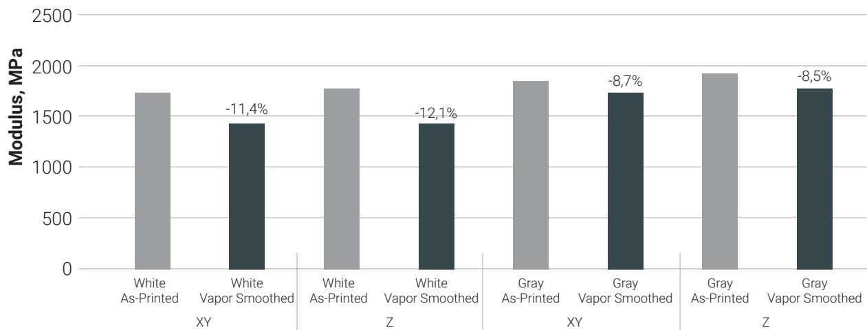
Figure 8: Young's Modulus Comparison
