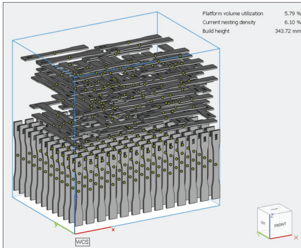
Figure 1: Test samples printing orientation
